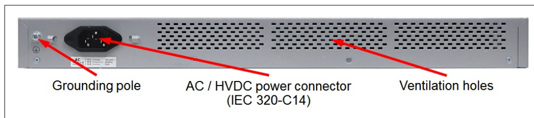
Figure 3. Rear panel of the CE0128T Switch
